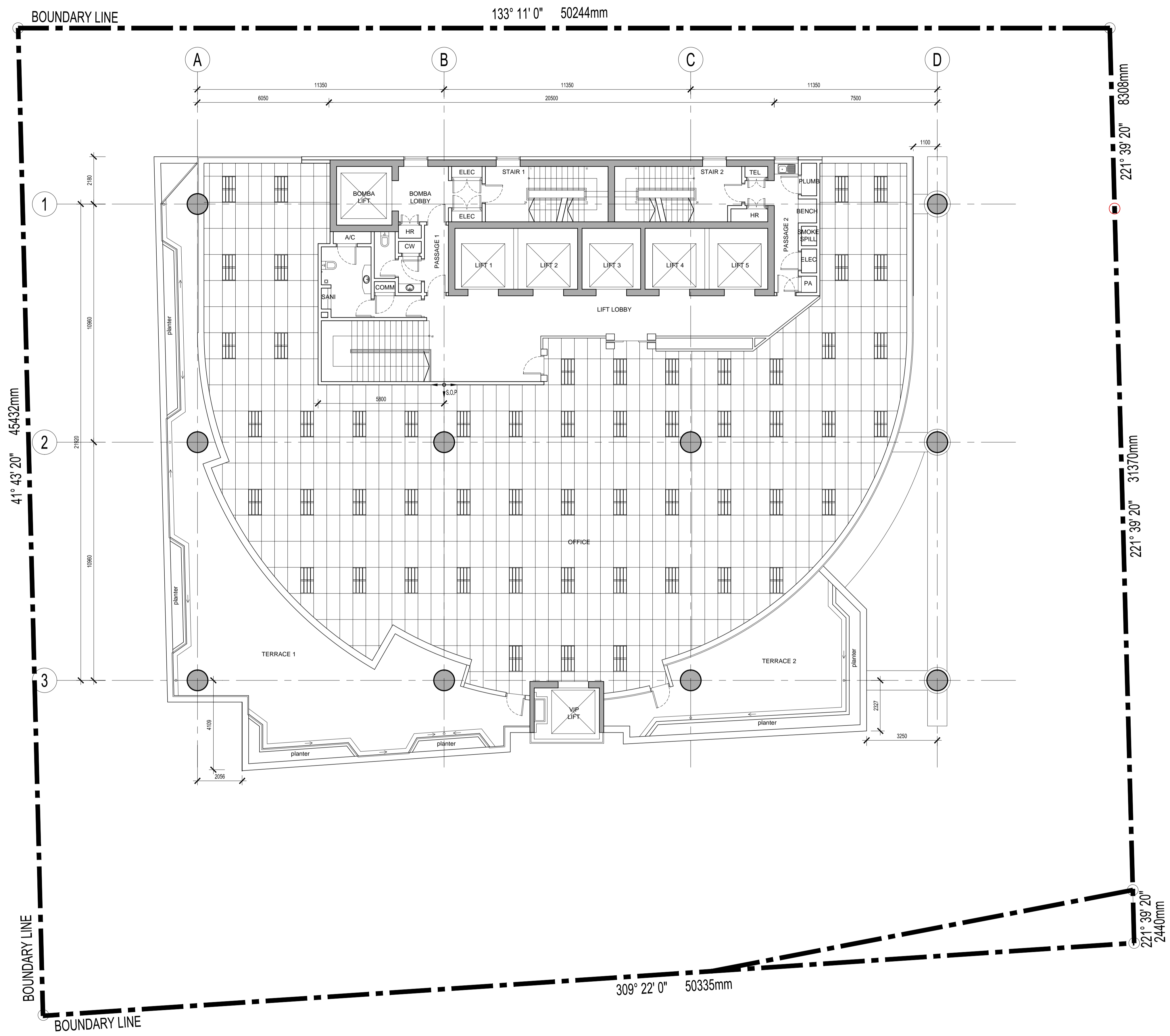
1. LEVEL 19 CEILING SETTING OUT POINT SCALE 1:100 @ A1
